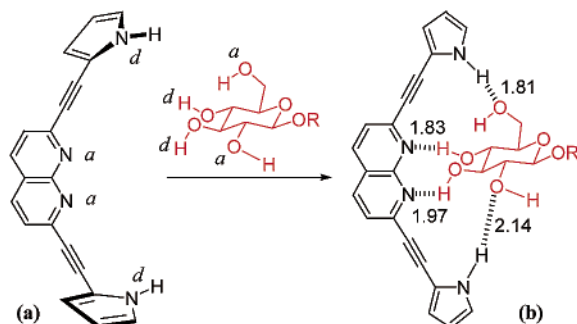
Figure 1. (a) Free BPN showing the conjugated daad array with two pyrrole rings slightly tilted toward opposite directions. (b) BPN and its associated BPN/ \beta -D-glucoside hydrogen-bonding complex. The geometrically optimized complex (R = CH 3 ) derived by the B3LYP/6-31G** method shows the distances (Å) of the hydrogen bonds.
